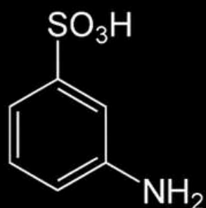
Metanilic Acid
