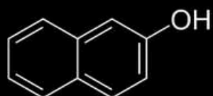
Beta Naphthol
